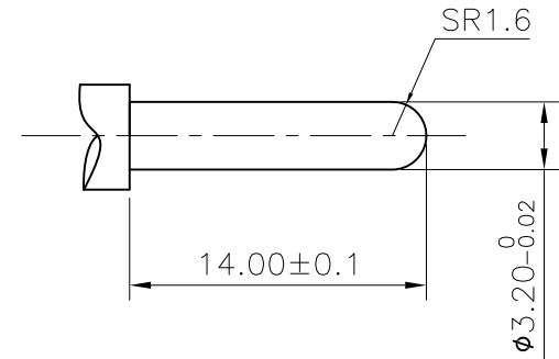
GAUGE PLUG:
