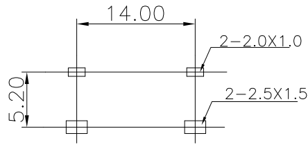
PCB LAYOUT TOP VIEW
