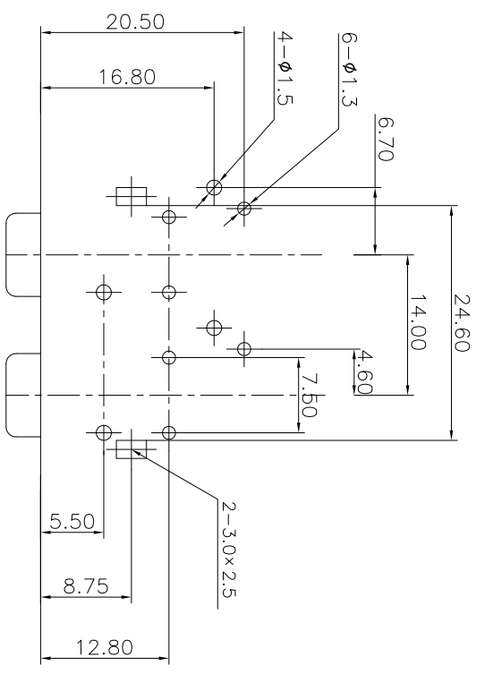
PCB LAYOUT TOP VIEW
