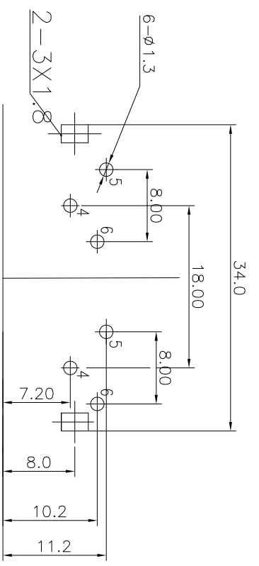
PCB LAYOUT TOP VIEW
